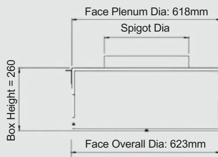
Diffuser with top entry
