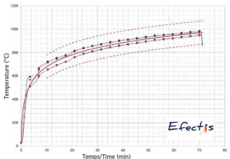
Fig 1: Furnace time/temperature graph showing fire test curve in accordance with EN1366-3:2021, detailed in EN 1363-1.
