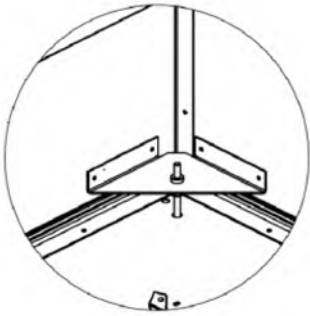
Plenum fixing bracket detail
